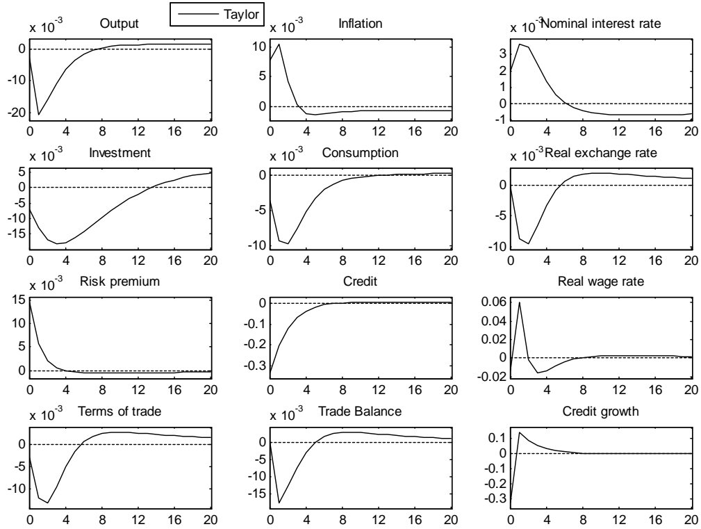
Fig. 3. Estimated IRFs for a premium shock
