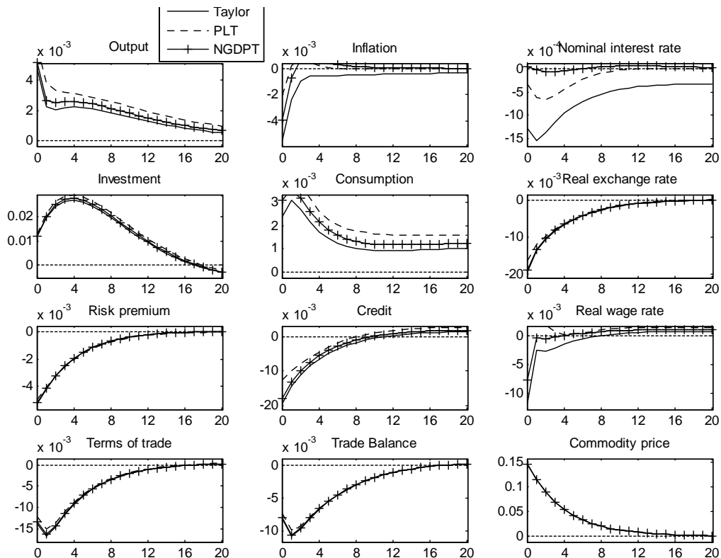
Fig. 6. Comparison of three monetary regimes IRFs to a commodity price shock
