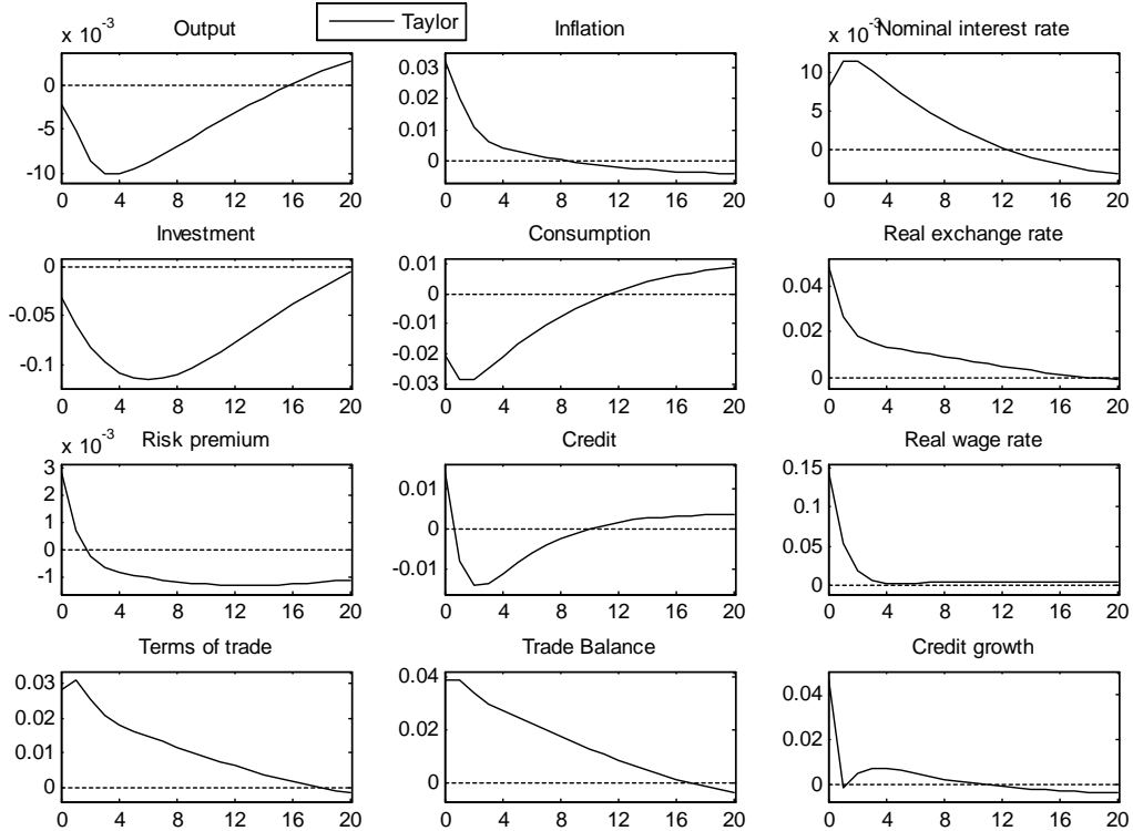
Fig. 4. Estimated IRFs for a foreign nominal interest rate shock
