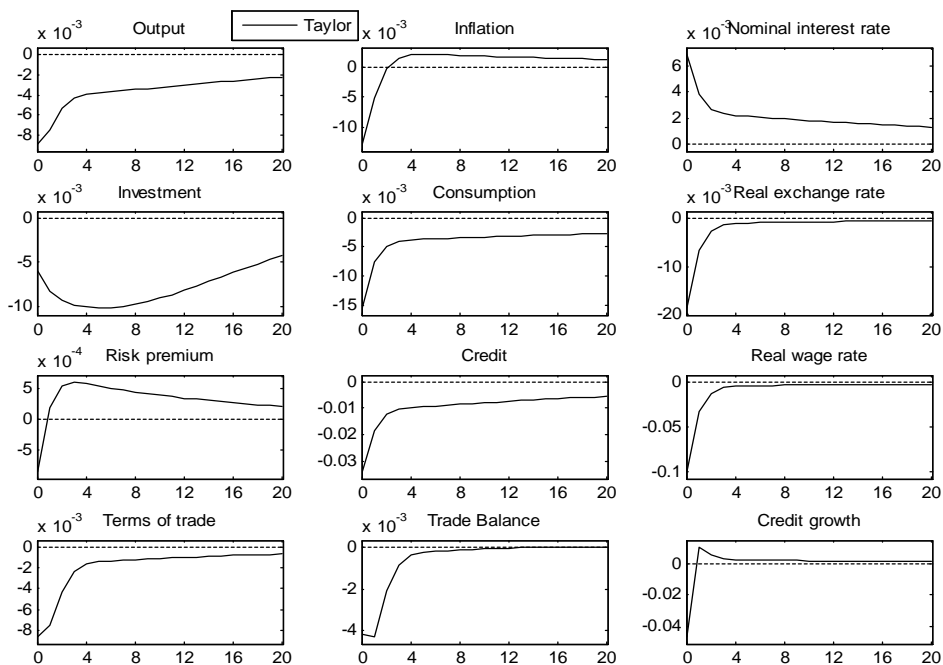
Fig. 2. Estimated IRFs for a monetary shock
