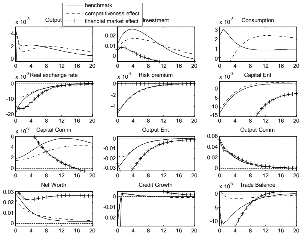
Fig. 5. Estimated IRFs and three channels of commodity price shock.
